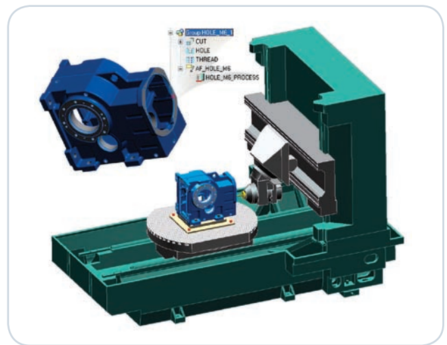
Capture manufacturing processes with manufacturing Annotation Features.
